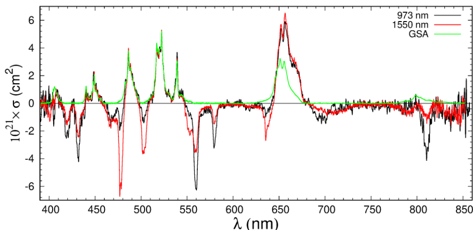
Fig. 1. Excited-state and ground-state absorption (GSA) spectra of Er:CaF_2:CdF_2 . The pump wavelengths are indicated by plot legend.
