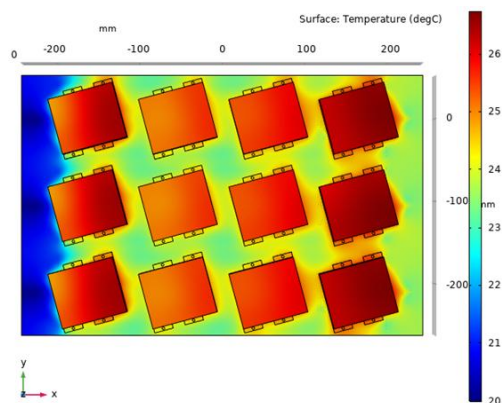
Fig. 1. Temperature distribution for optimized configuration showing ~1°C uniformity.
