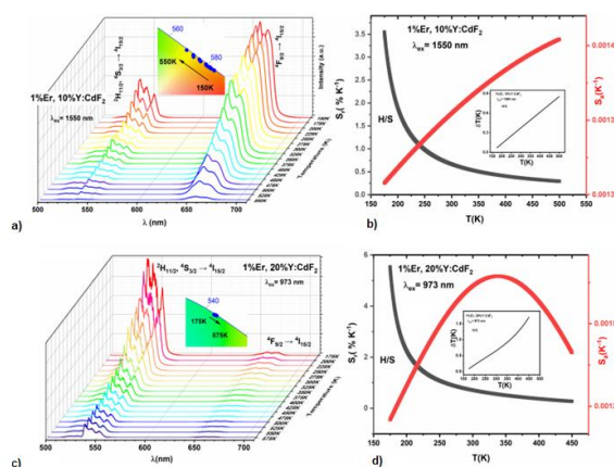
Fig. 1 Temperature dependence emission spectra of 1Er, 10Y under 1550 nm excitation (a) and 1Er, 20Y under 973 nm excitation (c) samples and their CIE chromaticity diagram as insets. The S_r and S_a curves, together with temperature uncertainty \delta T as insets (b, d).
