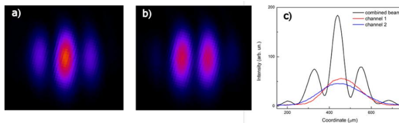
Fig. 1. Interference patterns corresponding to a) in-phase combination ( \Delta\phi = 0 ) and b) anti-phase combination ( \Delta\phi = \pi ).
