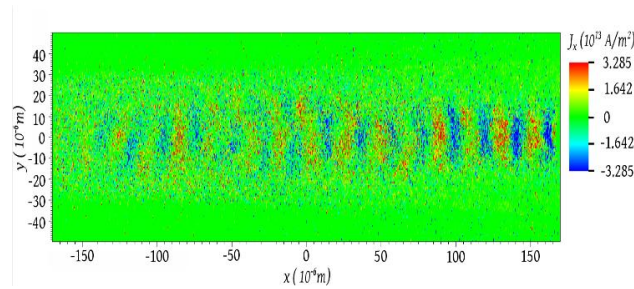
Fig. 1 Current distribution in a gas jet plasma irradiated by high intensity laser pulse.
