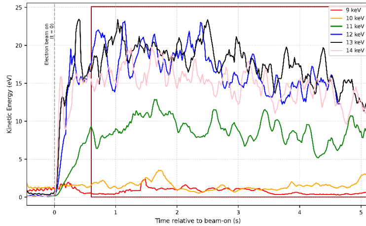
Fig. 1. Time evolution of the particles' kinetic energy for electron beam energies ranging from 9 to 14 keV. The electron beam is switched on at t = 0 [3].
