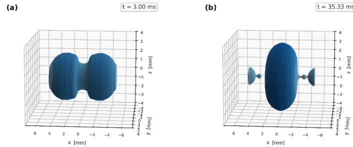
Fig. 1. 3D OpenFOAM simulation (interIsoFoam isoAdvector VOF, 5+5 mm water droplets, conical needle, 50 \mu\text{m} mesh). (a) Bridge growth phase at t = 3.00\text{ ms} , characteristic hourglass shape of the merging droplets. (b) Lamb shape oscillation after detachment from needles at t = 35.33\text{ ms} , small liquid caps remain pinned at the conical needle rims.
